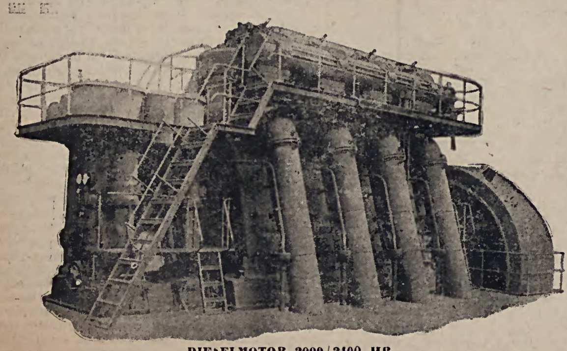
DISELMOTOR 2000/2100 HP.
