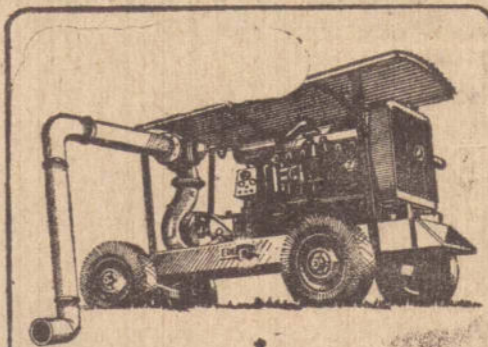
Moto Bomba Diesel com Motor Mercedes Benz 0 M 355 180 H.P. Bomba KSB 600 m 3 /h
