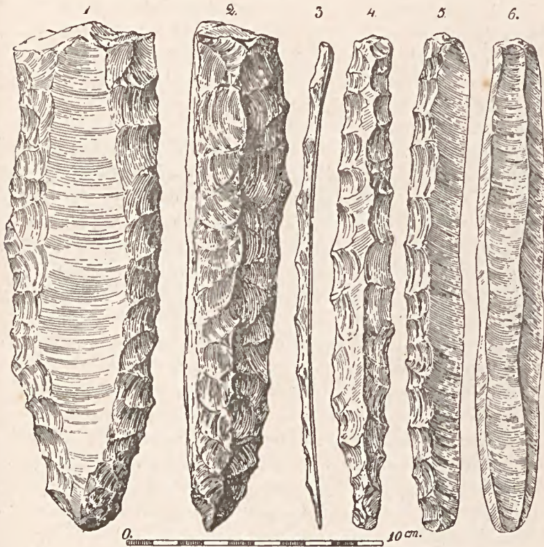
Fig. 70. — N o 1-2, nucleus (Grand-Pressigny). — N o 3-4, 1 re lame. N o 5, 2 e lame. — N o 6, 2 e lame.
